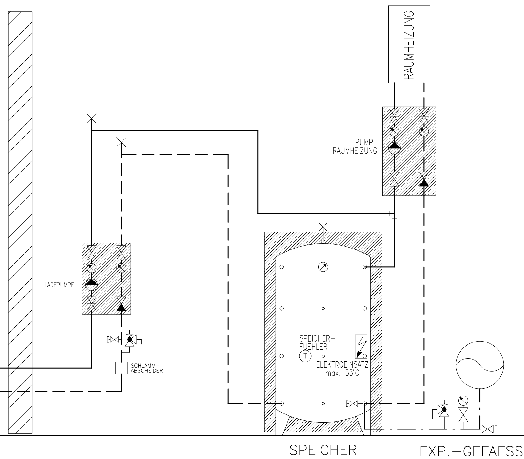
WAERMEPUMPE DIMPLEX LA 60P-TUR
